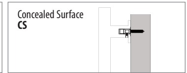
Optional Mounting
