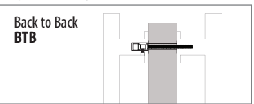
Optional Mounting
