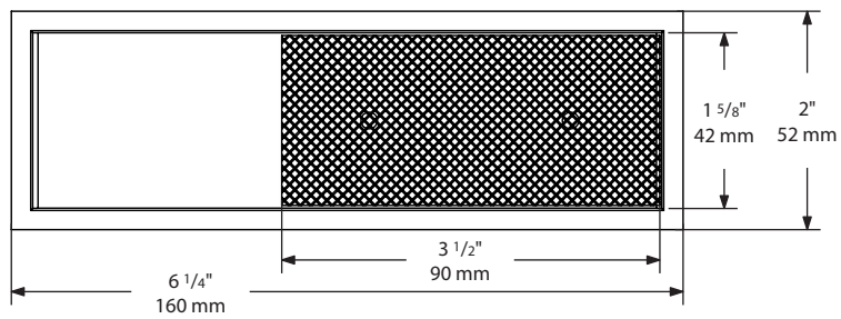
FRONT VIEW
