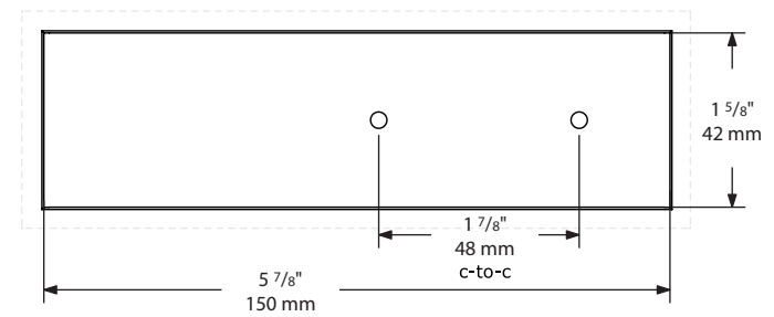
BACK VIEW
